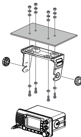
Overhead Mounting
